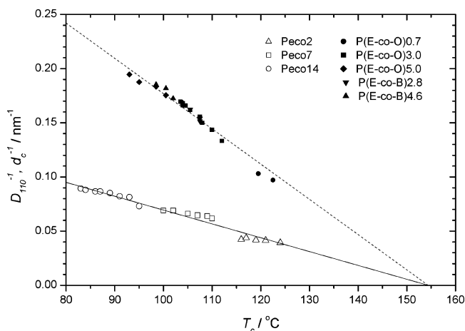
Figure 1. Different samples PEc(O/B) x crystallized at various temperatures T_c : crystallization line d_c^{-1} vs T_c determined by SAXS (from ref 10) and lateral coherence lengths D_{110} derived from the line width of the 110 reflection (open symbols).
