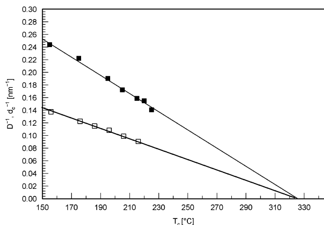
Figure 3. iPS crystallized at various temperatures T_c : crystallization line d_c^{-1} vs T_c determined by SAXS (from ref 8) and lateral coherence lengths D_{200} derived from the line width of the 200 reflection (open circles).
