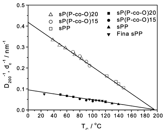
Figure 2. Different samples of sPP (sPP, sP(P-co-O) x , and the commercial Fina sPP) crystallized at various temperatures T_c : crystallization line d_c^{-1} vs T_c determined by SAXS (from ref 7) and lateral coherence lengths D_{200} derived from the line width of the 200 reflection (filled symbols).
